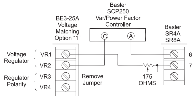
Figure 12 - Basler SRA Interconnection
