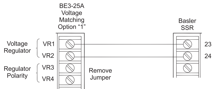
Figure 13 - Basler SSR Interconnection
