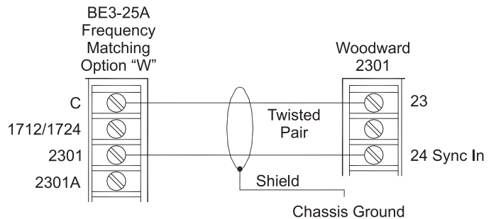
Figure 5 - Woodward 2301 Interconnection
