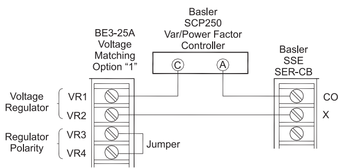
Figure 11 - Basler SSE, SER-CB Interconnection
