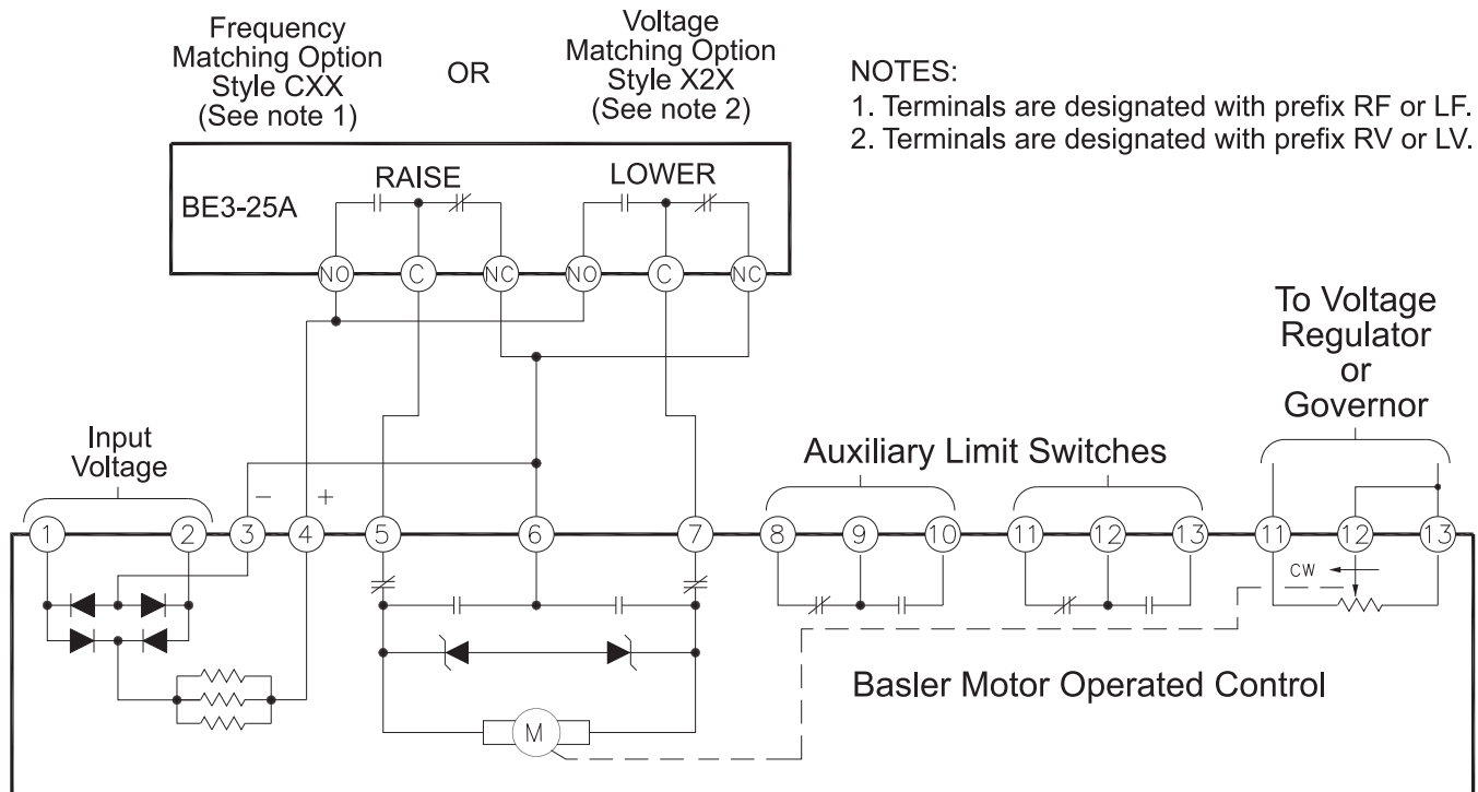
Figure 8 - Raise/Lower Contact Interconnection
