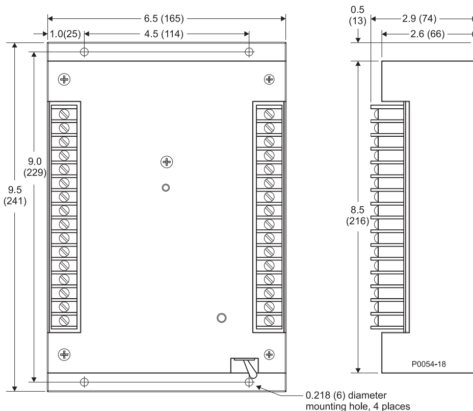
Figure 18 - Outline Drawing
