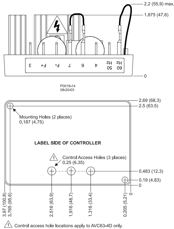
Figure 6 - Outline and Drilling Drawing
